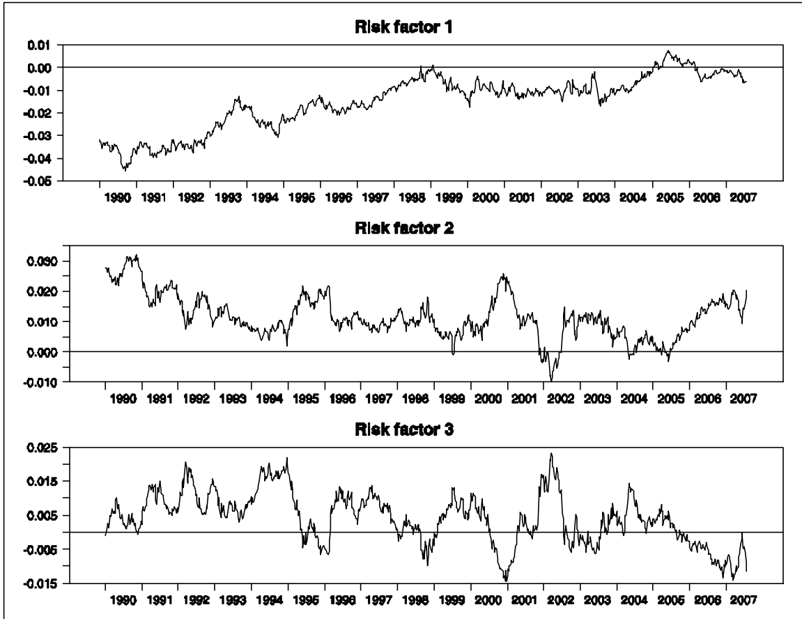
Figure 6. Values of the three elements of \Sigma I_t , weekly from Jan 5, 1990 to July 27, 2007.
