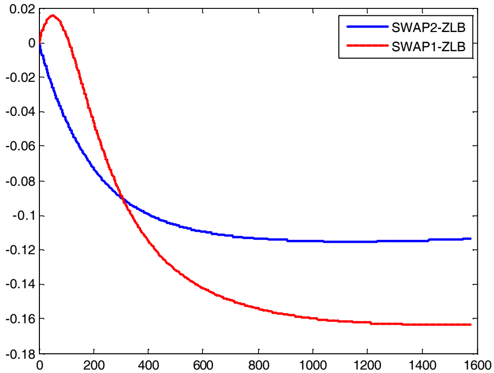
Figure 13. Effects of two different maturity swaps when implemented at the zero lower bound. Dashed curve: Fed sells all its holdings of less than 1-year maturity and retires debt at the longest end of the maturity structure (plot of 5200b_n^* f\Delta as a function of n ). Solid curve: Fed sells all its holdings of less than 1-year maturity and retire debt evenly across 2-1/2 to 10 year maturities (plot of 5200b_n^* f\Delta_2 ).
