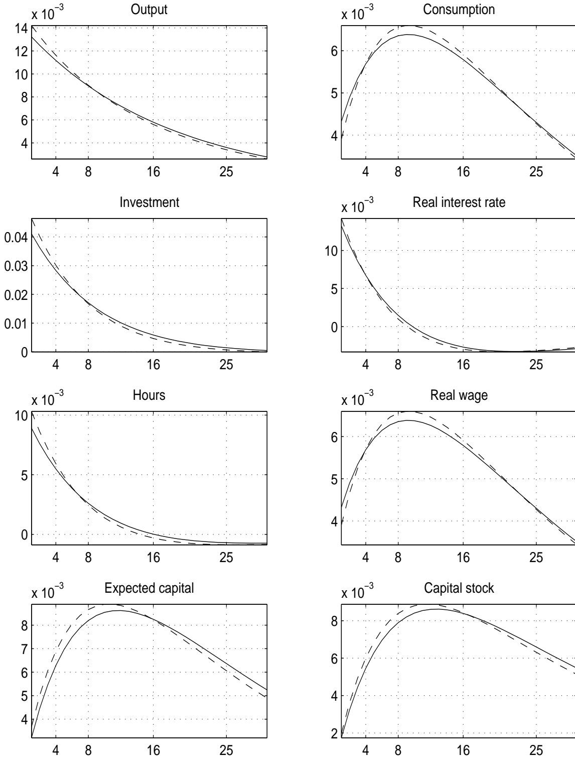
FIGURE 4. Model with alternative learning rule ( g = 0.001 and t_0 = 10000 ): Impulse responses to a neutral technology shock. The solid line represents the responses under rational expectations. The dashed line represents the responses under adaptive expectations.
