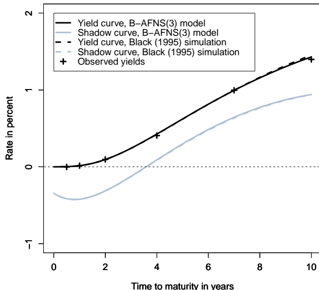
Figure 4: Fitted Yield Curves in Three-Factor Shadow-Rate Models. Fitted and shadow yield curves from an option-based estimated B-AFNS(3) model are shown as of January 9, 2004. In addition, the corresponding curves are shown based on a simulation using Black’s (1995) approach and N = 25,000 paths of the state variables drawn using the option-based estimated B-AFNS(3) model factor dynamics under the Q -measure.
