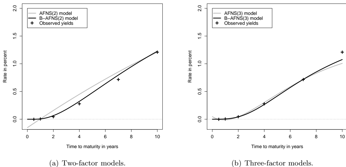
Figure 6: Fitted Yield Curves on July 1, 2005. The figure to the left illustrates the fitted yield curves from the AFNS(2) and B-AFNS(2) models on July 1, 2005. Also shown are the six observed yields on that date. The figure to the right shows the corresponding results for the AFNS(3) and B-AFNS(3) models.
