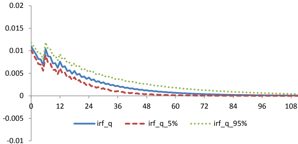
Figure 1. The impulse response function (IRF) in months of the real exchange rate to a one standard-deviation shock during the pre-euro and euro periods, respectively, based on the bias-corrected CCEP estimates of the autoregression equation (2) reported in Table 1. Dashed lines are 5% and 95% confidence intervals, constructed using the double bootstrap method of Kilian (1998) with 2000 iterations.
