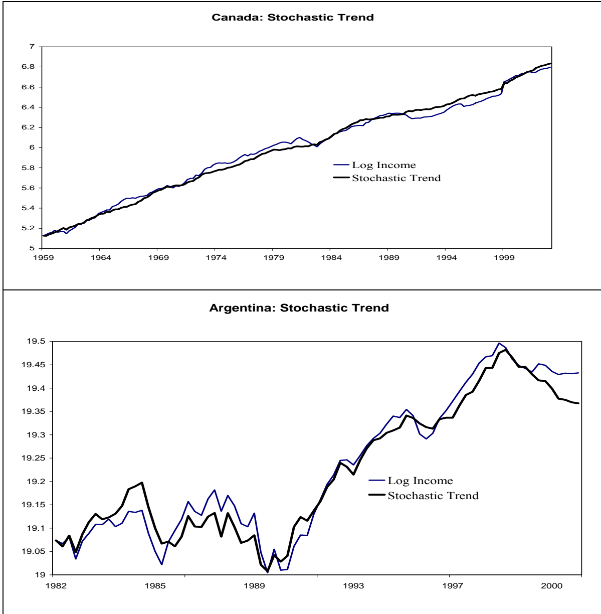
Figure 1: Stochastic Trends estimated using the KPSW(1991) methodology
