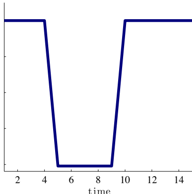
Output gap
