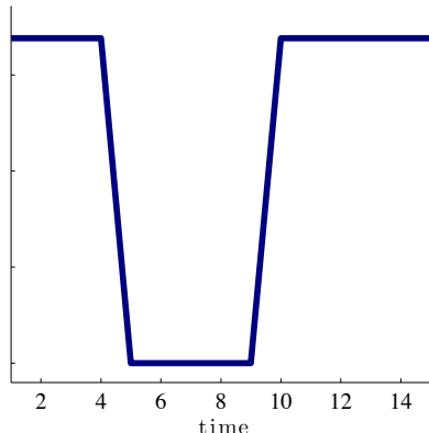
Nominal rate
