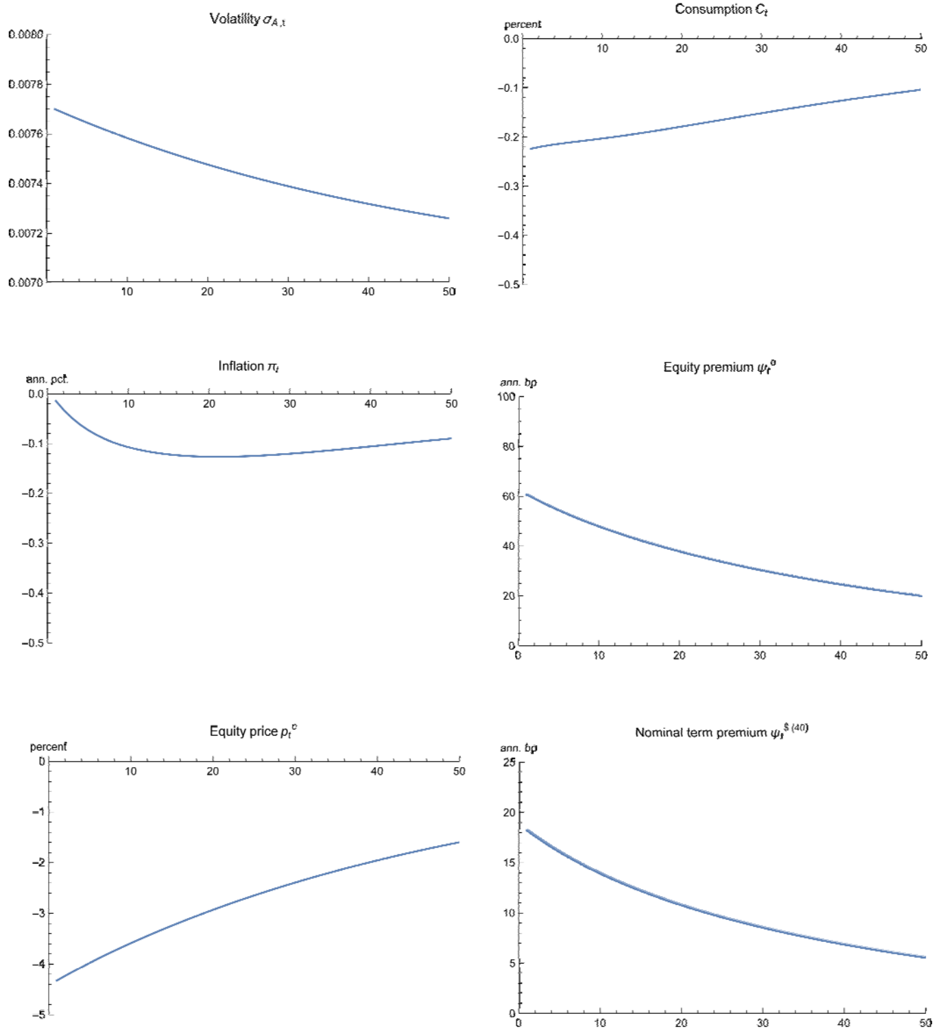
Figure 9. Nonlinear impulse response functions for volatility \sigma_t^A , consumption C_t , inflation \pi_t , the equity premium \psi_t^e , equity price p_t^e , and nominal term premium \psi_t^{s(40)} to a one-standard-deviation (0.1 percent, or .0007) positive volatility shock in the extended model. See text for details.
