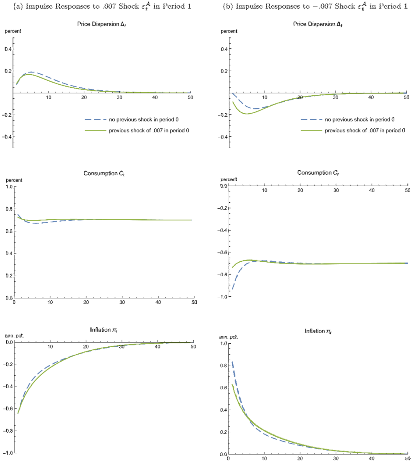
Figure 7. Comparison of nonlinear impulse response functions for price dispersion \Delta_t , consumption C_t , and inflation \pi_t to a one-standard-deviation (0.7 percent) (a) positive vs. (b) negative technology shock in period 1. Dashed blue lines depict impulse response functions relative to a baseline of no previous shocks, with state variables initialized to their nonstochastic steady-state values, as in previous figures. Solid green lines depict impulse response functions relative to a different baseline, after a positive 0.7 percent technology shock in period 0. The figure shows that the conditional volatility of prices and consumption are lower after a positive 0.7 percent technology shock in period 0, particularly in response to negative shocks in period 1. See text for details.
