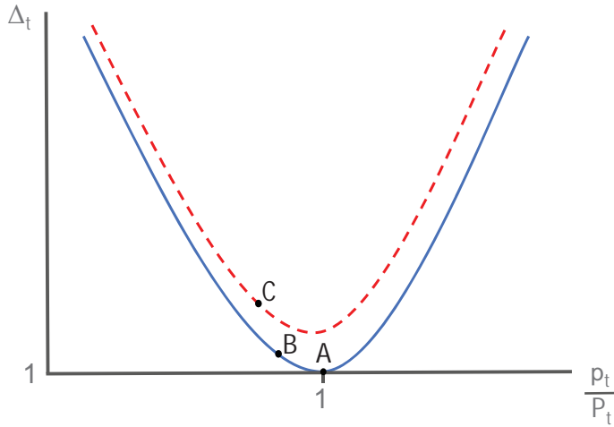
Figure 8. Illustrative graph of price dispersion \Delta_t as a function of monopolistic firms' time- t reset price p_t/P_t . The solid blue line assumes p_\tau/P_\tau = 1 for all \tau < t ; the dashed red line assumes p_{t-1}/P_{t-1} < 1 and p_\tau/P_\tau = 1 for all \tau < t-1 . Point A denotes firms' risk-neutral optimal price (or the optimal price in the linearized model), point B denotes firms' risk-averse optimal price, and point C firms' risk-averse optimal price after p_{t-1}/P_{t-1} < 1 . See text for details.
