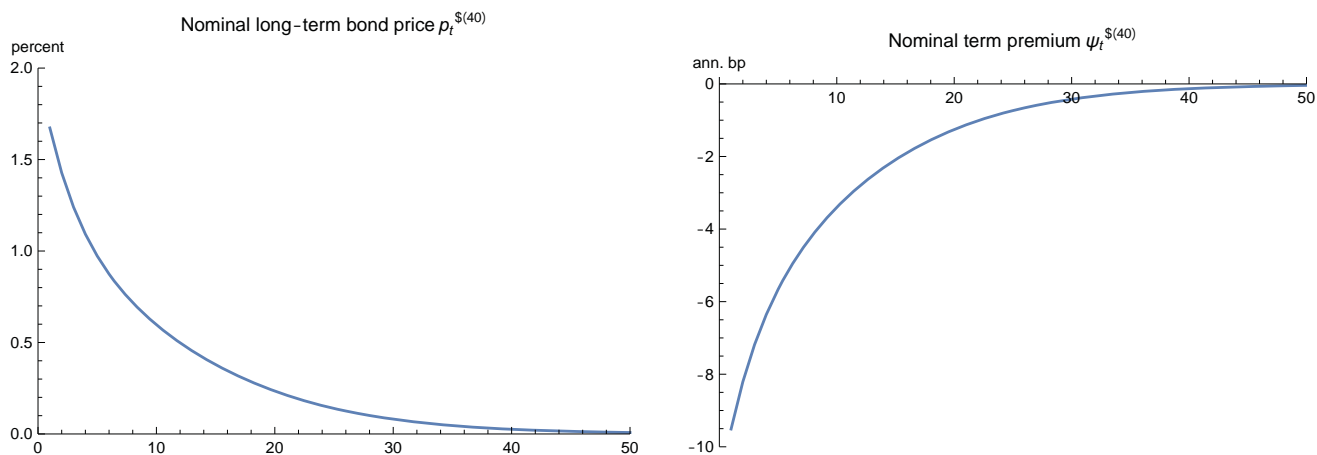
Figure 4. Nonlinear impulse response functions for nominal long-term bond price p_t^{\$(40)} and term premium \psi_t^{\$(40)} to a one-standard-deviation (0.7 percent) technology shock in the model, with state variables initialized to their nonstochastic steady state values. See text for details.
